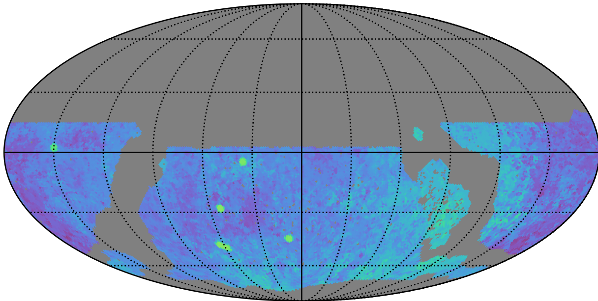
noroll_mjdp0_v3.4_10yrs WFD g band: Median Season Length
