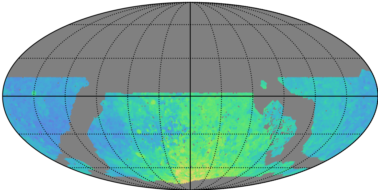
noroll_mjdp0_v3.4_10yrs WFD all bands: Median Season Length
