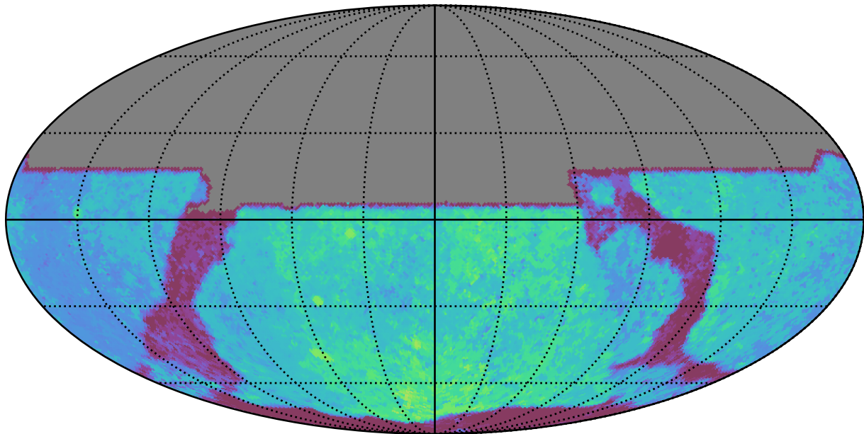
noroll_mjdp0_v3.4_10yrs All sky y band: Median Season Length
