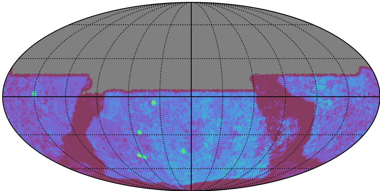
noroll_mjdp0_v3.4_10yrs All sky u band: Median Season Length
