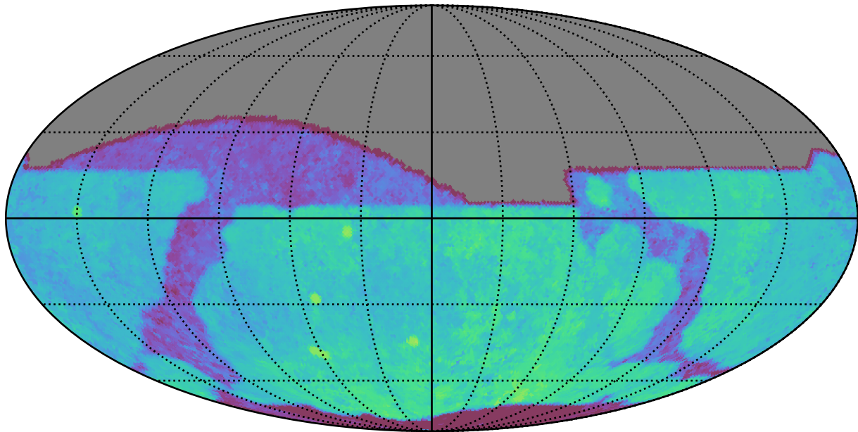
noroll_mjdp0_v3.4_10yrs All sky r band: Median Season Length
