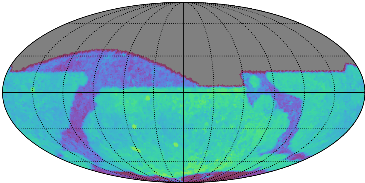
noroll_mjdp0_v3.4_10yrs All sky i band: Median Season Length
