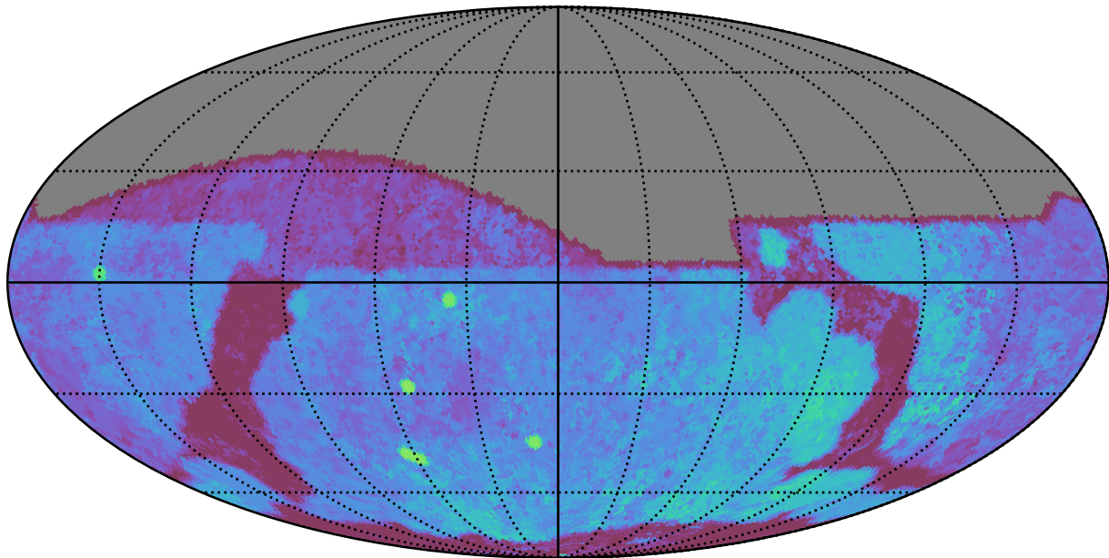
noroll_mjdp0_v3.4_10yrs All sky g band: Median Season Length
