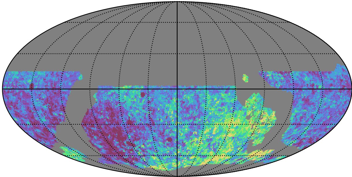
noroll_mjdp0_v3.4_10yrs WFD z band: Median Inter-Night Gap
