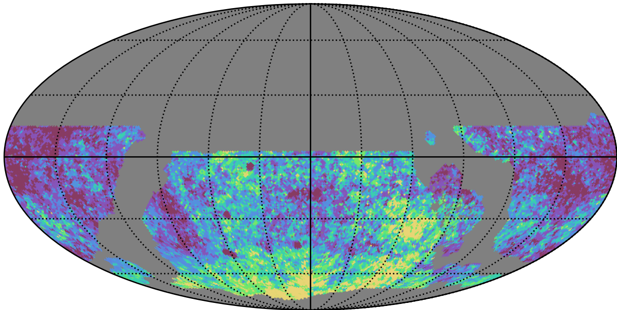
noroll_mjdp0_v3.4_10yrs WFD r band: Median Inter-Night Gap
