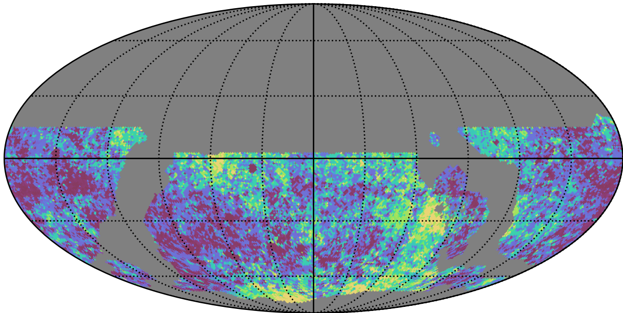
noroll_mjdp0_v3.4_10yrs WFD i band: Median Inter-Night Gap
