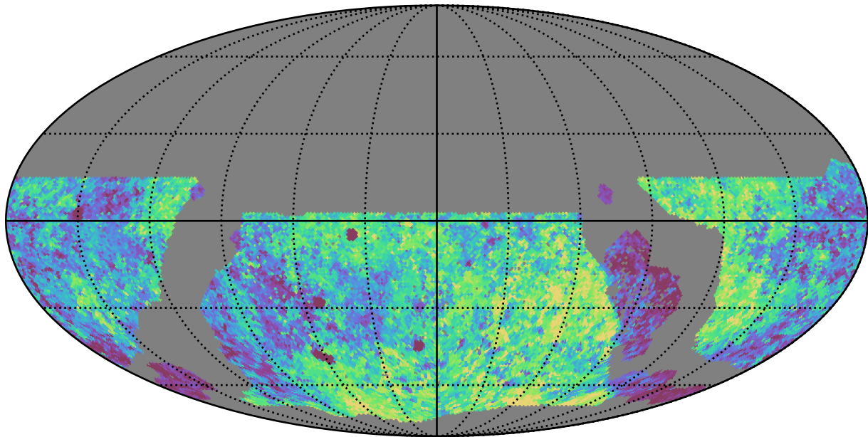
noroll_mjdp0_v3.4_10yrs WFD g band: Median Inter-Night Gap
