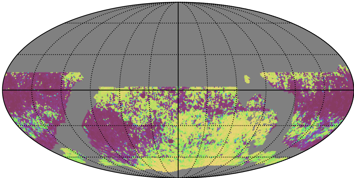
noroll_mjdp0_v3.4_10yrs WFD all bands: Median Inter-Night Gap
