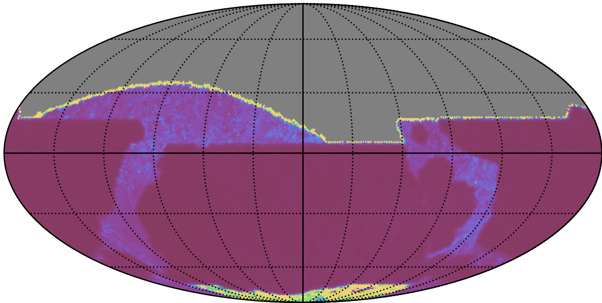
noroll_mjdp0_v3.4_10yrs All sky z band: Median Inter-Night Gap
