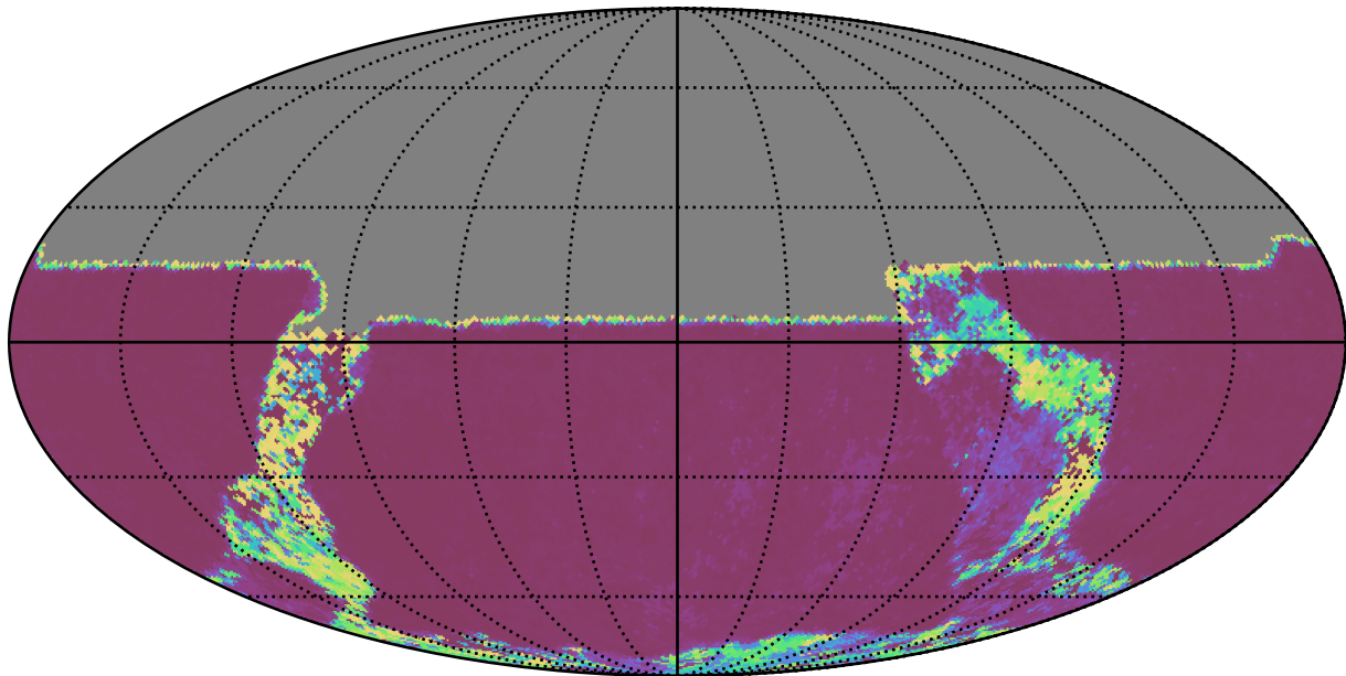
noroll_mjdp0_v3.4_10yrs All sky u band: Median Inter-Night Gap
