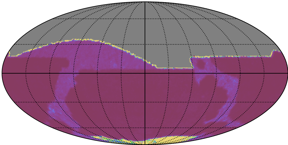
noroll_mjdp0_v3.4_10yrs All sky r band: Median Inter-Night Gap
