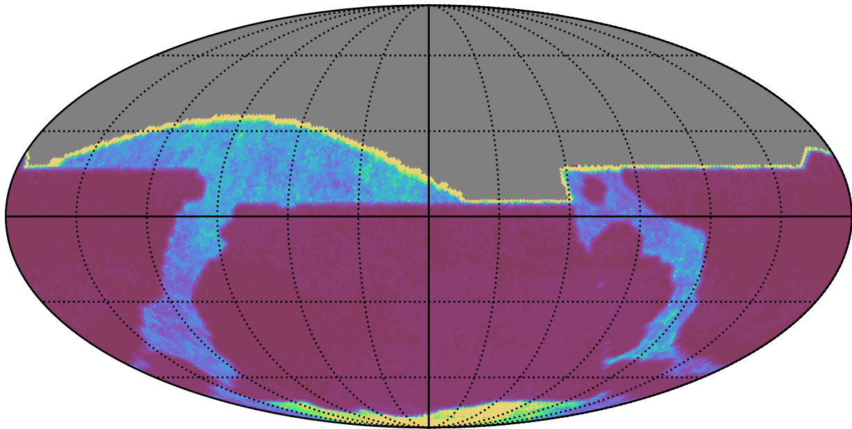
noroll_mjdp0_v3.4_10yrs All sky all bands: Median Inter-Night Gap
