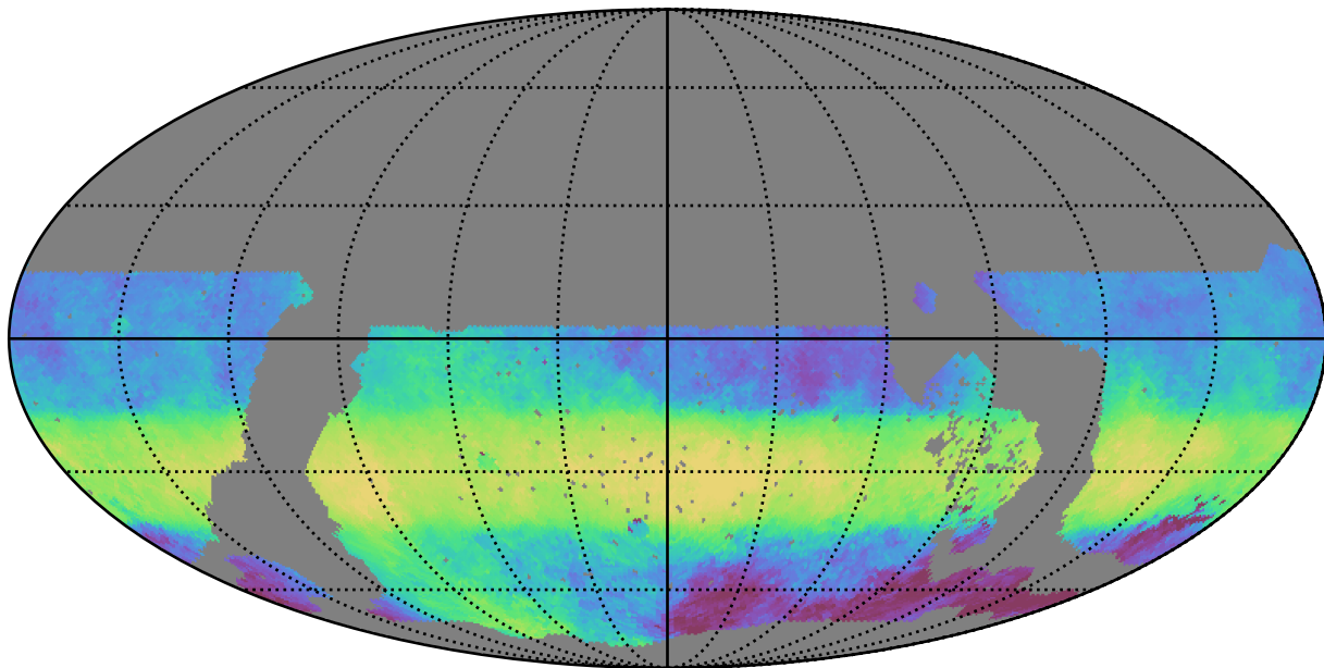
noroll_mjdp0_v3.4_10yrs WFD z band: Median HA
