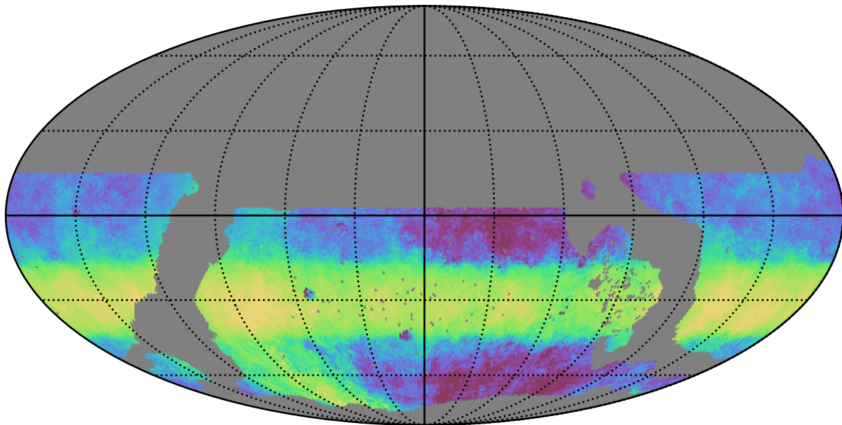
noroll_mjdp0_v3.4_10yrs WFD y band: Median HA
