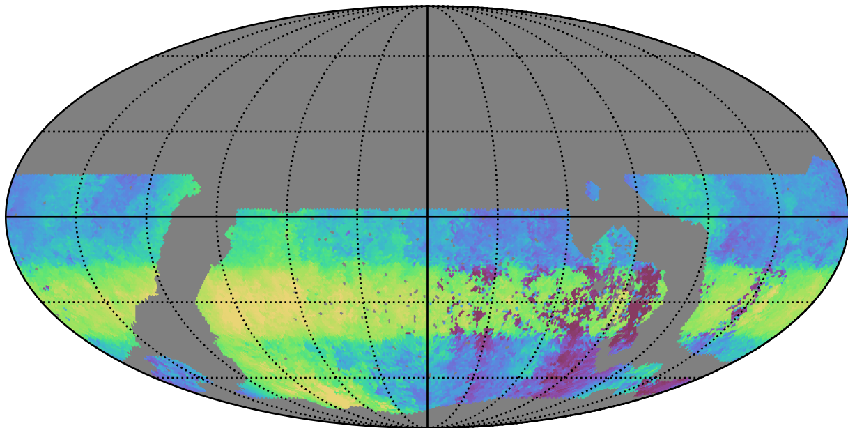
noroll_mjdp0_v3.4_10yrs WFD u band: Median HA
