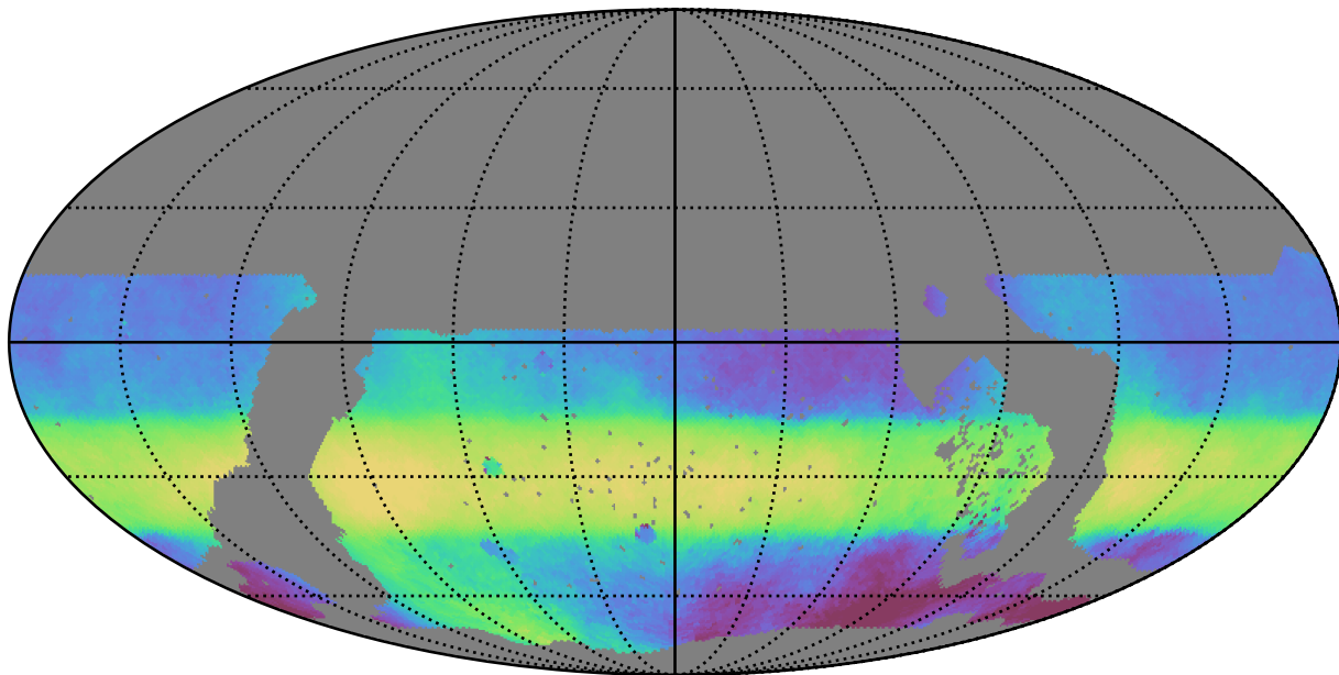
noroll_mjdp0_v3.4_10yrs WFD all bands: Median HA
