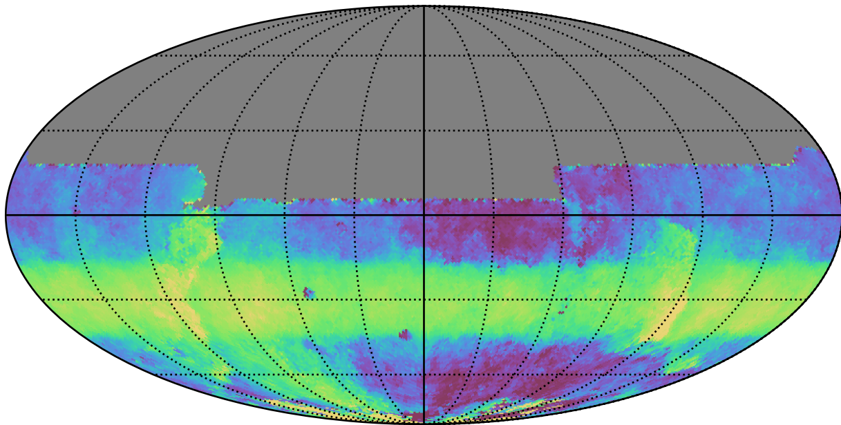
noroll_mjdp0_v3.4_10yrs All sky y band: Median HA
