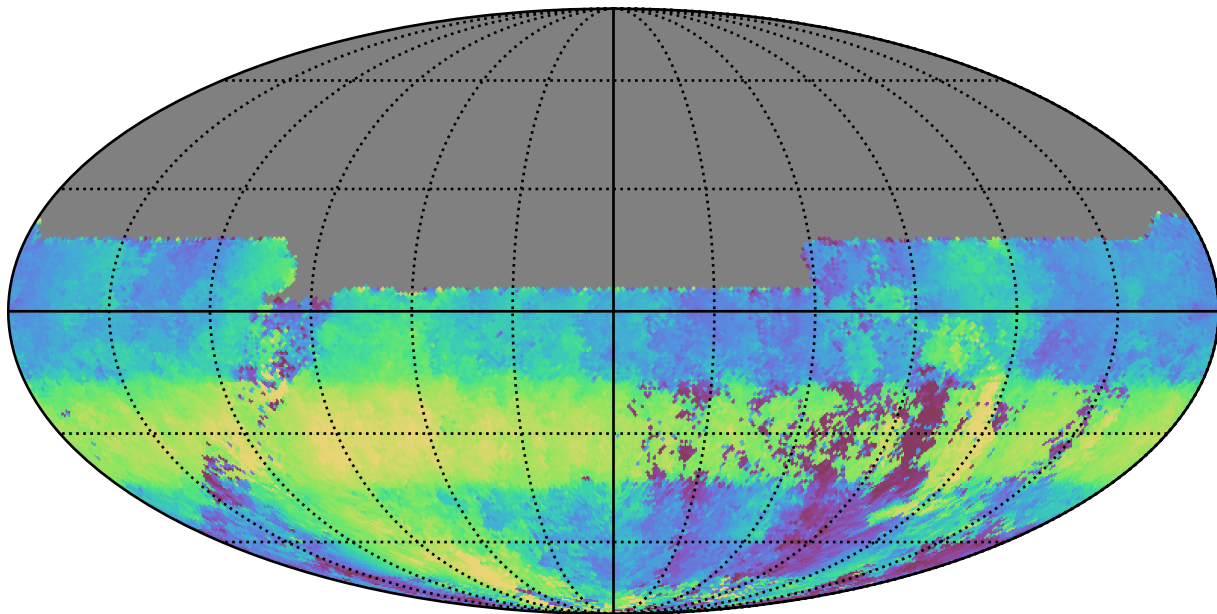
noroll_mjdp0_v3.4_10yrs All sky u band: Median HA
