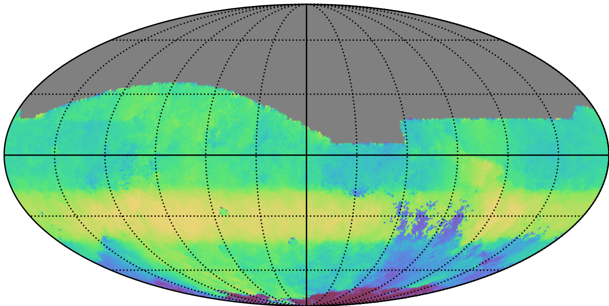
noroll_mjdp0_v3.4_10yrs All sky r band: Median HA
