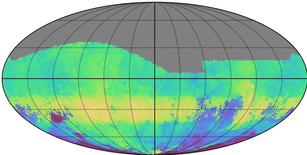
noroll_mjdp0_v3.4_10yrs All sky g band: Median HA
