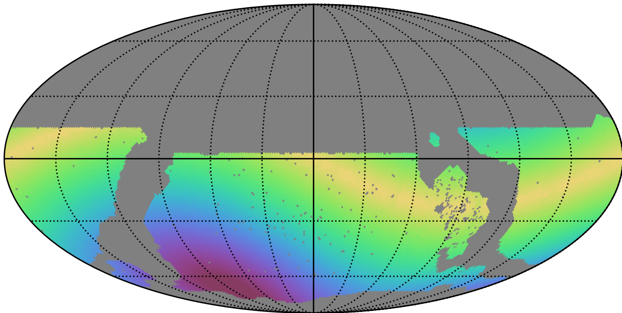
noroll_mjdp0_v3.4_10yrs WFD z band: Max solarElong
