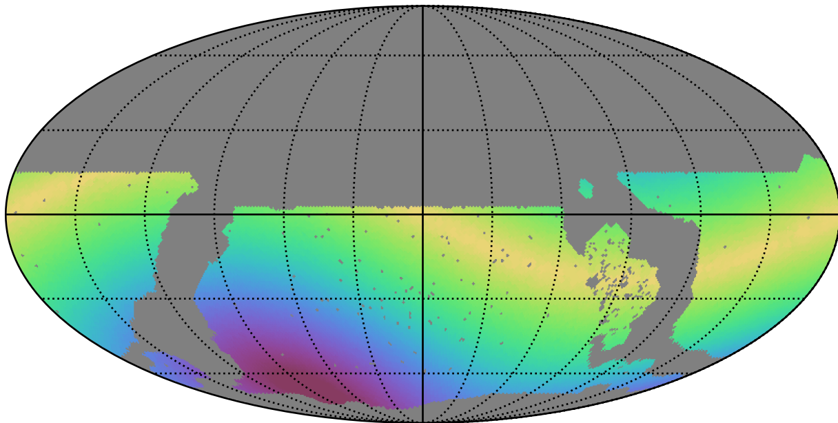
noroll_mjdp0_v3.4_10yrs WFD y band: Max solarElong
