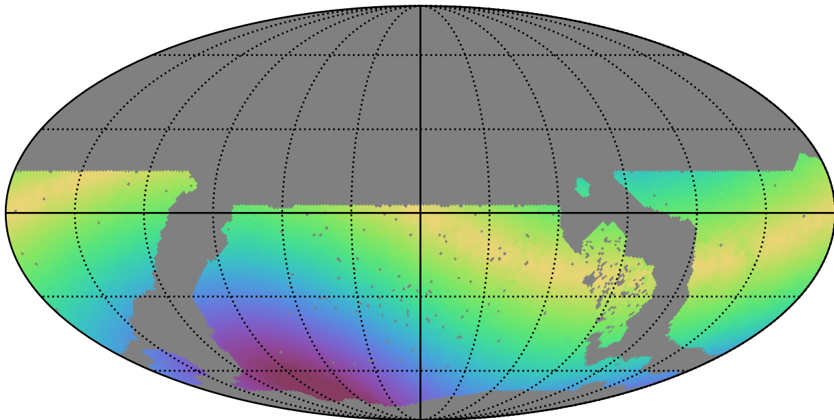
noroll_mjdp0_v3.4_10yrs WFD u band: Max solarElong
