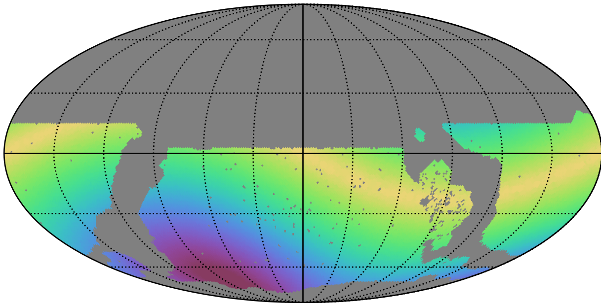
noroll_mjdp0_v3.4_10yrs WFD r band: Max solarElong
