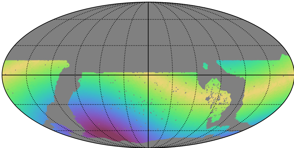
noroll_mjdp0_v3.4_10yrs WFD g band: Max solarElong
