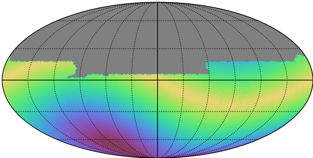
noroll_mjdp0_v3.4_10yrs All sky y band: Max solarElong
