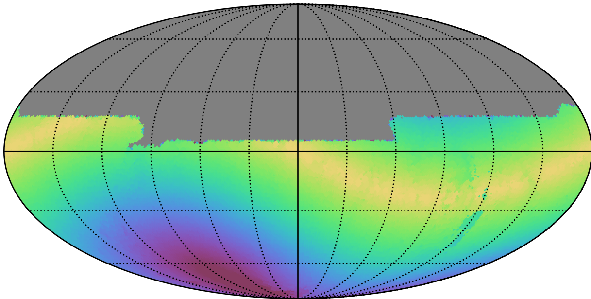
noroll_mjdp0_v3.4_10yrs All sky u band: Max solarElong
