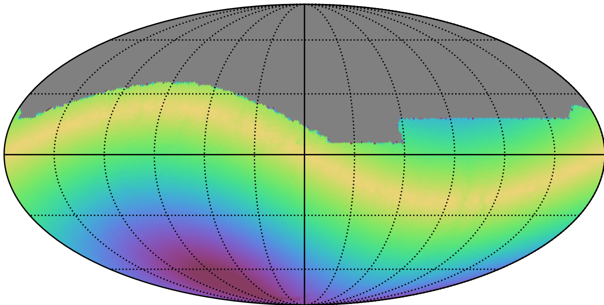
noroll_mjdp0_v3.4_10yrs All sky i band: Max solarElong
