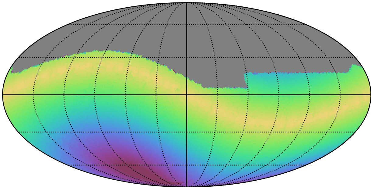
noroll_mjdp0_v3.4_10yrs All sky g band: Max solarElong
