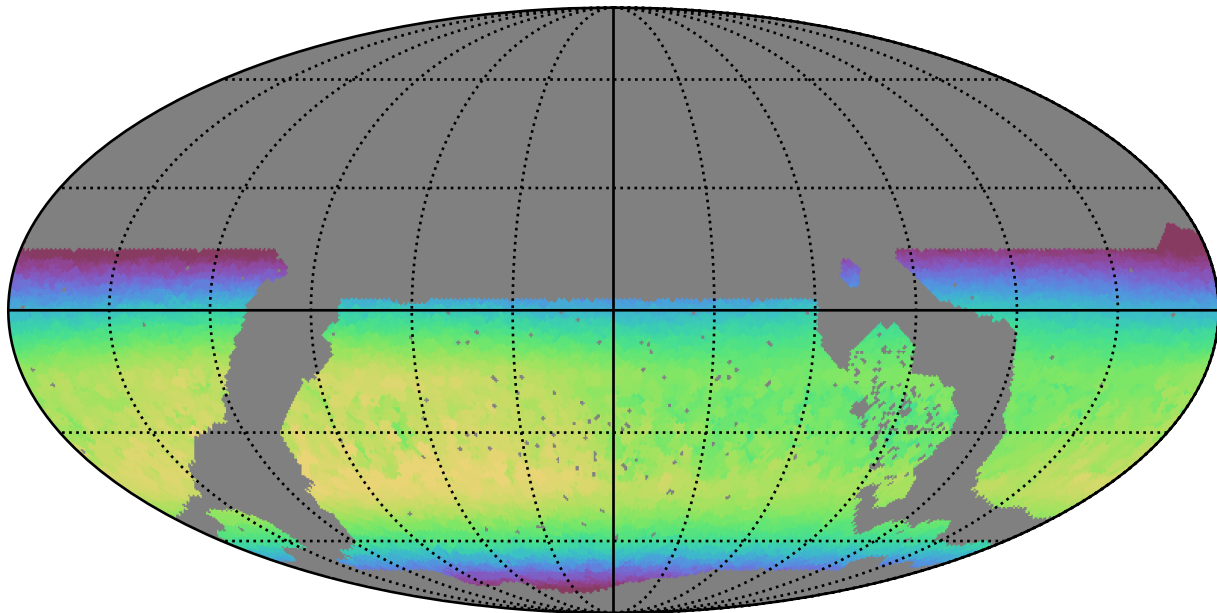
noroll_mjdp0_v3.4_10yrs WFD z band: Max skyBrightness
