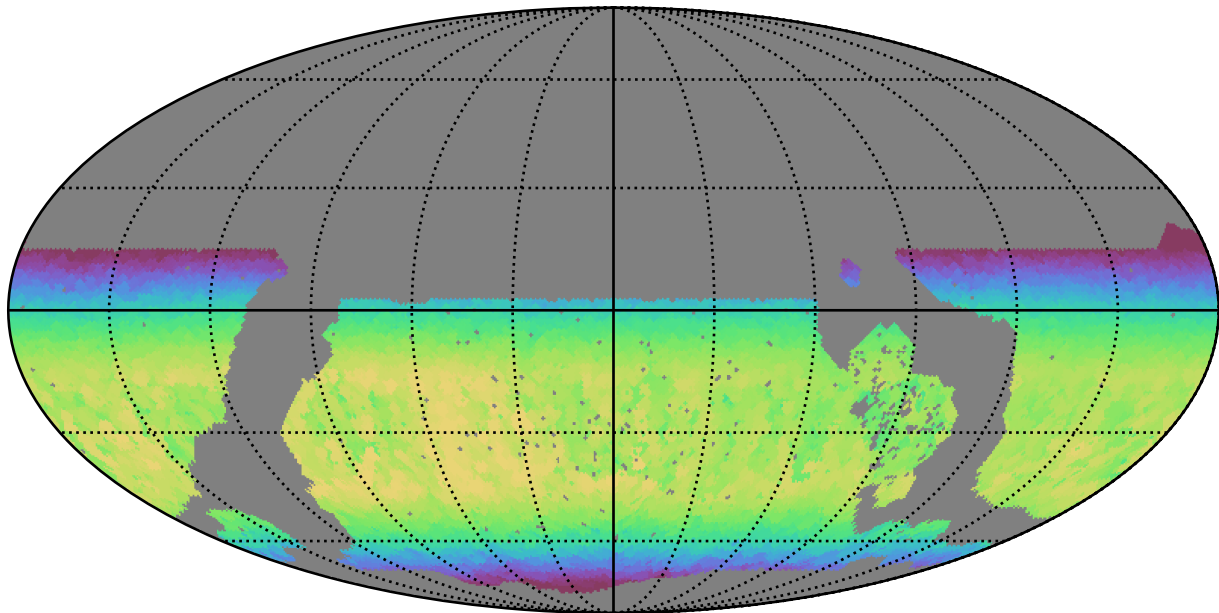
noroll_mjdp0_v3.4_10yrs WFD y band: Max skyBrightness
