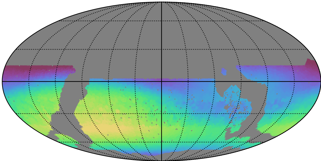
noroll_mjdp0_v3.4_10yrs WFD u band: Max skyBrightness
