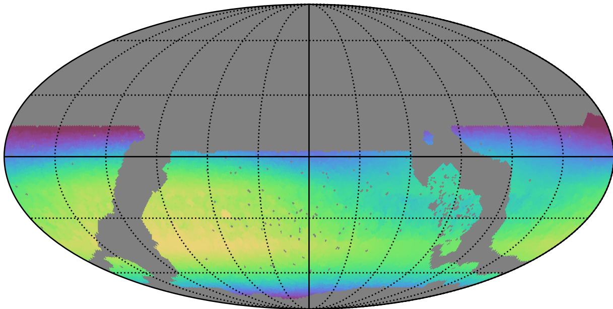
noroll_mjdp0_v3.4_10yrs WFD i band: Max skyBrightness
