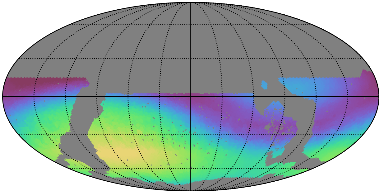
noroll_mjdp0_v3.4_10yrs WFD g band: Max skyBrightness
