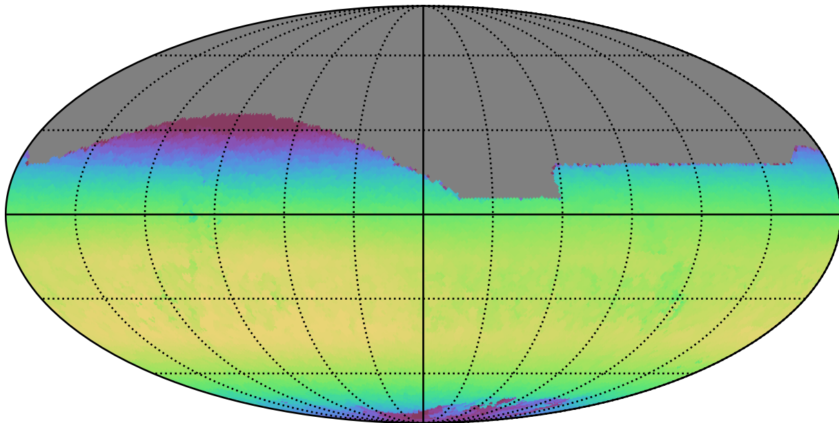
noroll_mjdp0_v3.4_10yrs All sky z band: Max skyBrightness
