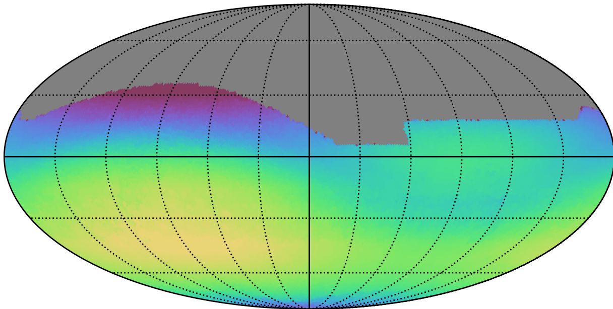
noroll_mjdp0_v3.4_10yrs All sky r band: Max skyBrightness
