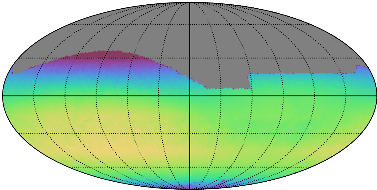
noroll_mjdp0_v3.4_10yrs All sky i band: Max skyBrightness
