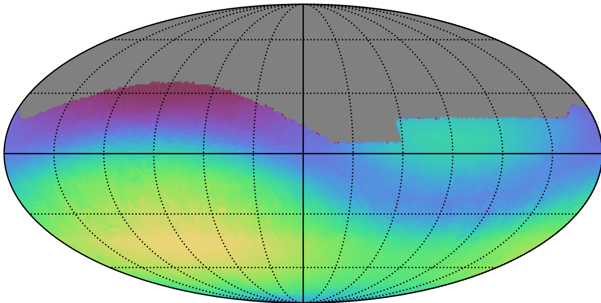
noroll_mjdp0_v3.4_10yrs All sky g band: Max skyBrightness
