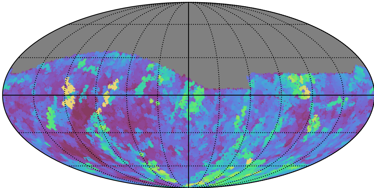
noroll_mjdp0_v3.4_10yrs Yr 1 r band: Max seeingGeom
