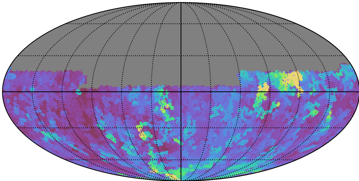
noroll_mjdp0_v3.4_10yrs Yr 1 u band: Max seeingEff
