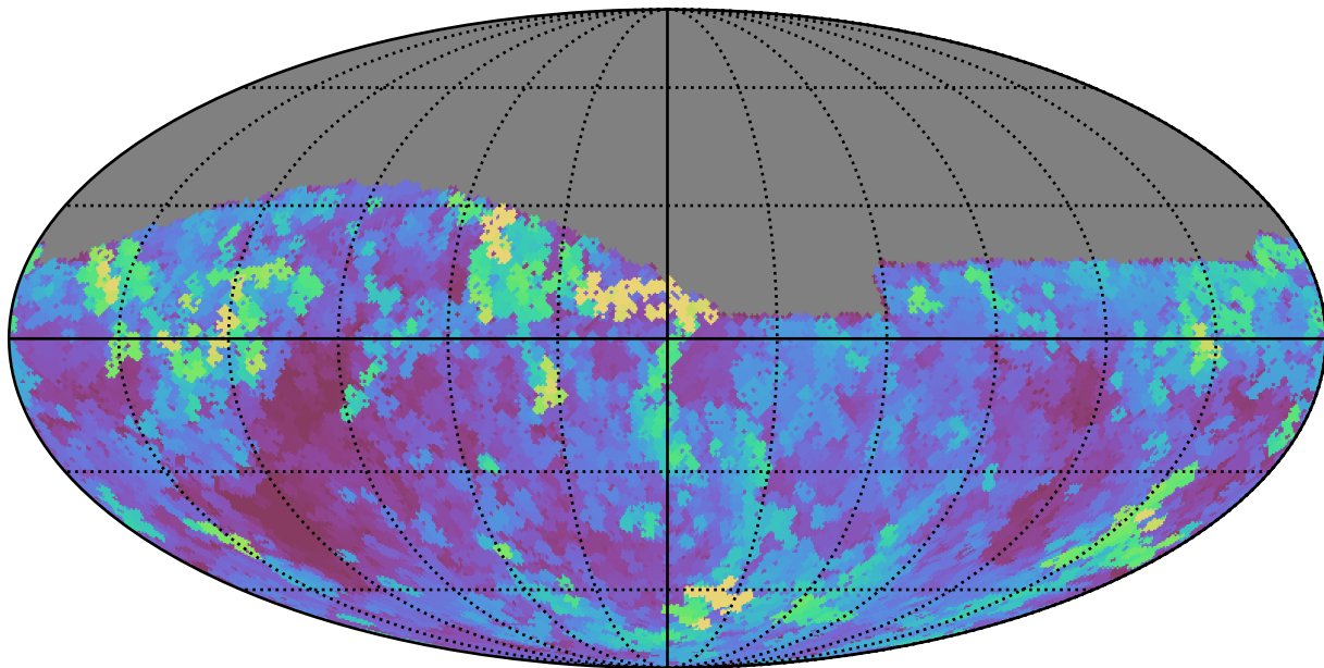
noroll_mjdp0_v3.4_10yrs Yr 1 i band: Max seeingEff
