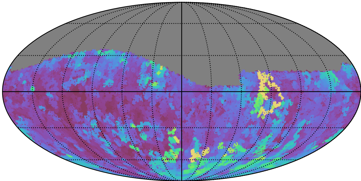
noroll_mjdp0_v3.4_10yrs Yr 1 g band: Max seeingEff
