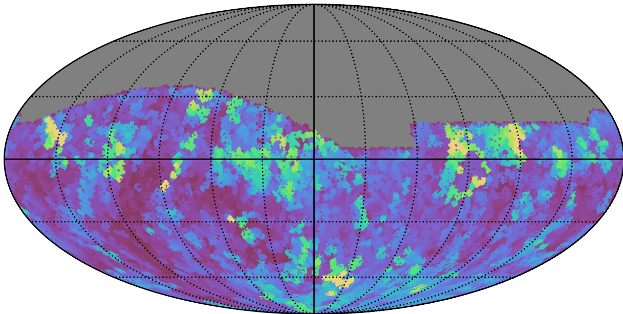
noroll_mjdp0_v3.4_10yrs Yr 1 all bands: Max seeingEff
