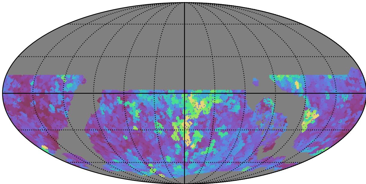
noroll_mjdp0_v3.4_10yrs WFD y band: Max seeingEff
