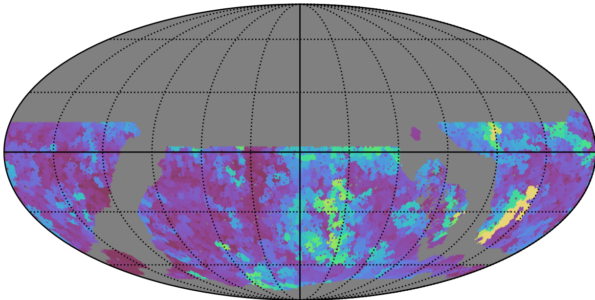
noroll_mjdp0_v3.4_10yrs WFD u band: Max seeingEff
