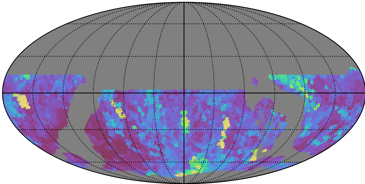
noroll_mjdp0_v3.4_10yrs WFD i band: Max seeingEff
